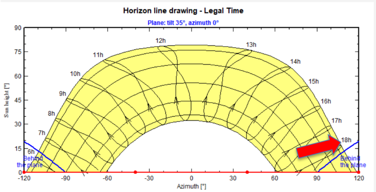
Figure 2: Horizon Line Drawing for Eager, AZ
