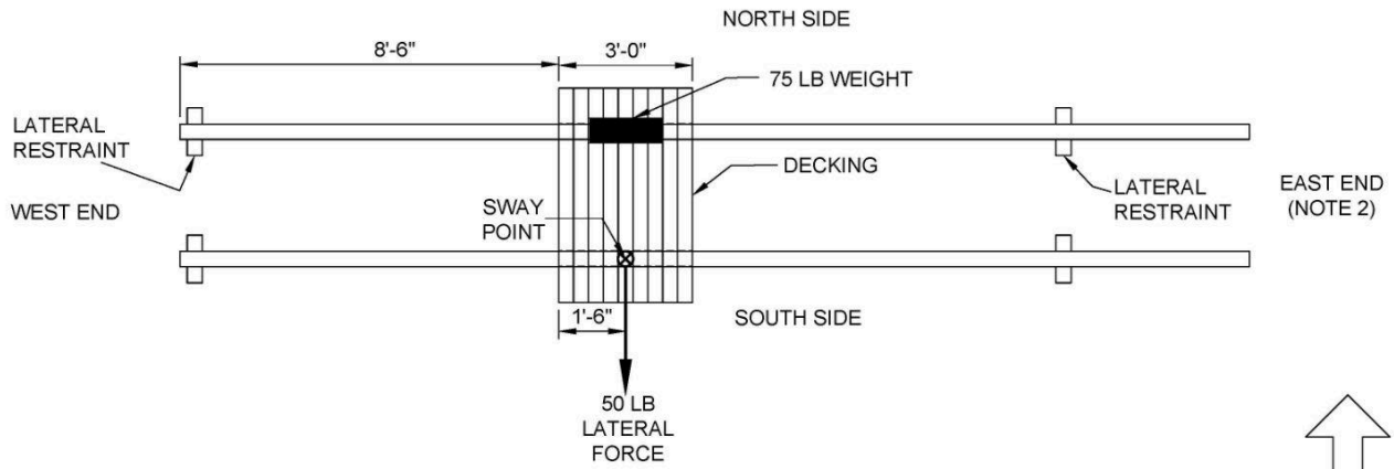
LATERAL LOAD TEST OF BACK SPAN
