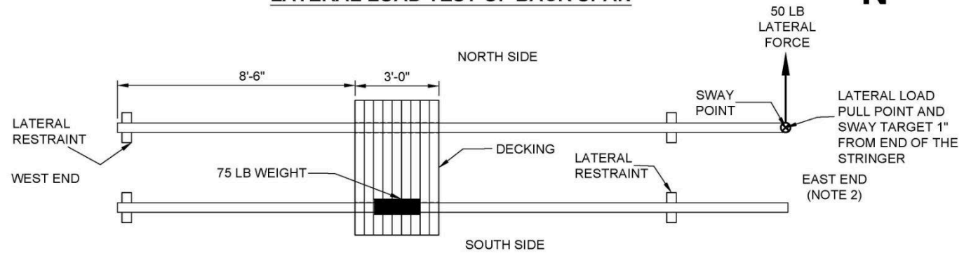
LATERAL LOAD TEST OF BACK SPAN
