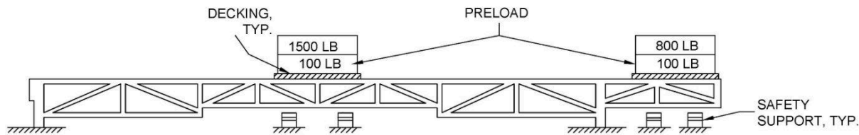
VERTICAL LOAD TEST ELEVATION
