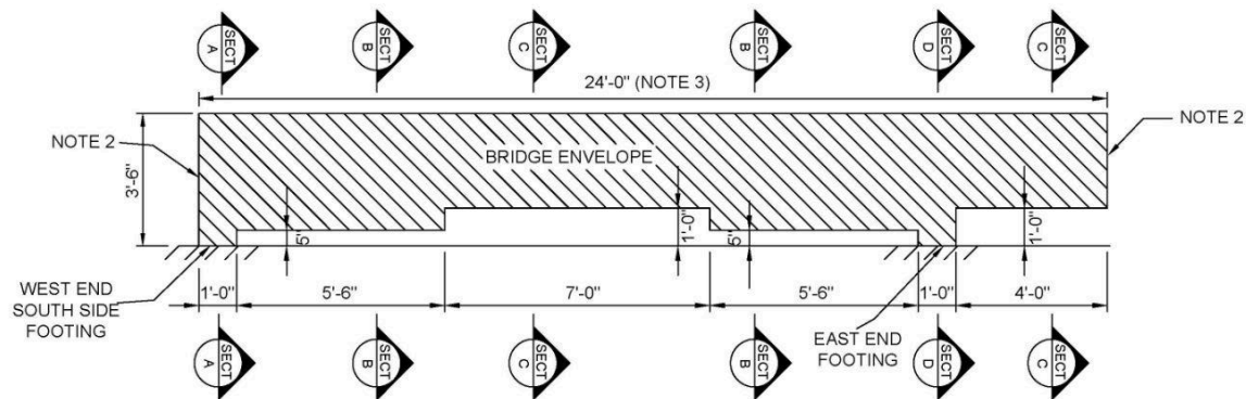
SOUTH SIDE ELEVATION
