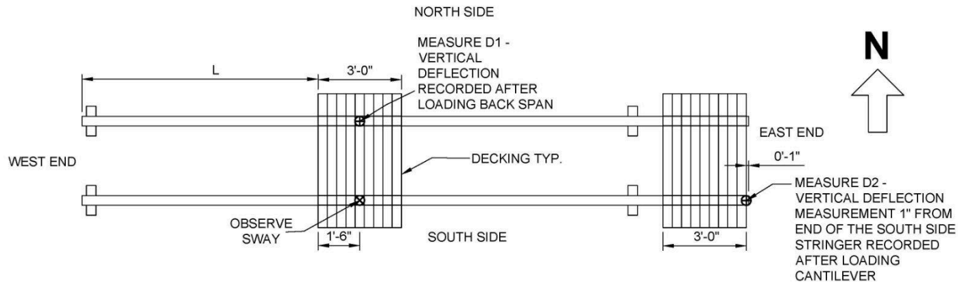
VERTICAL LOAD TEST PLAN
