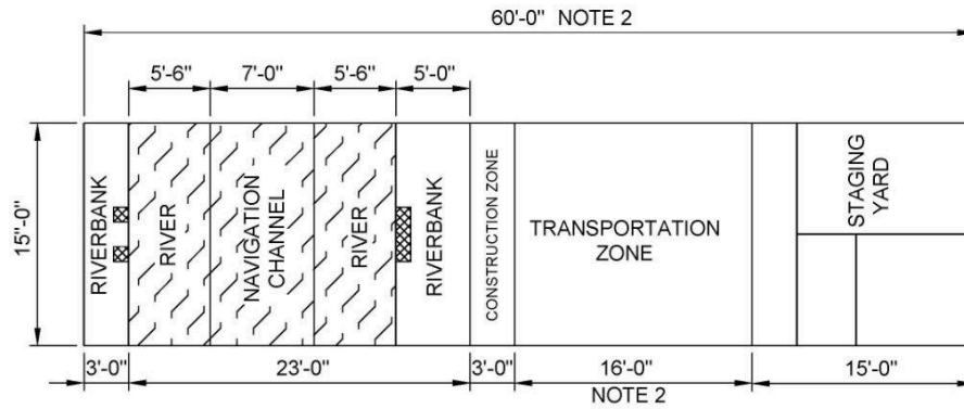
CONSTRUCTION SITE PLAN
