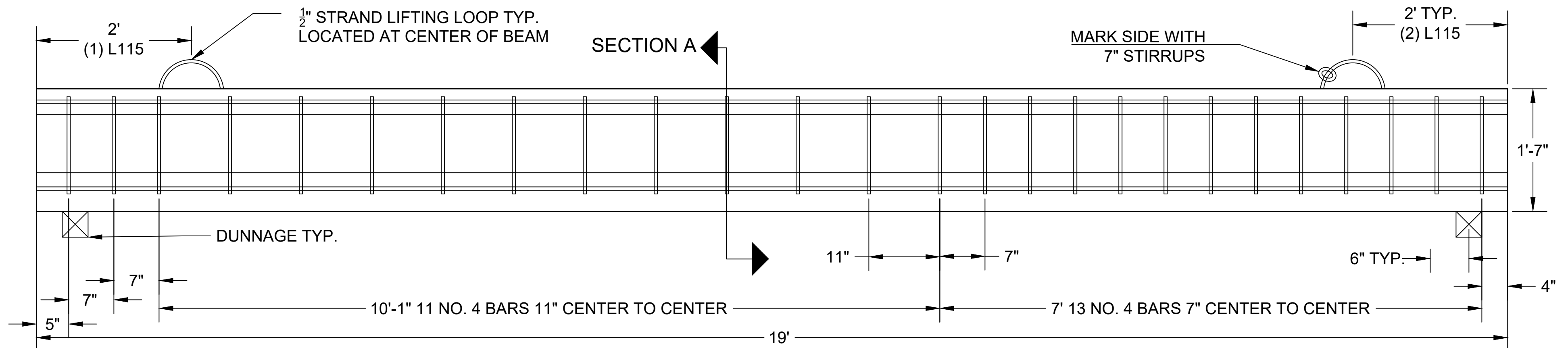
2 ELEVATION VIEW SCALE: 1" = 12"
